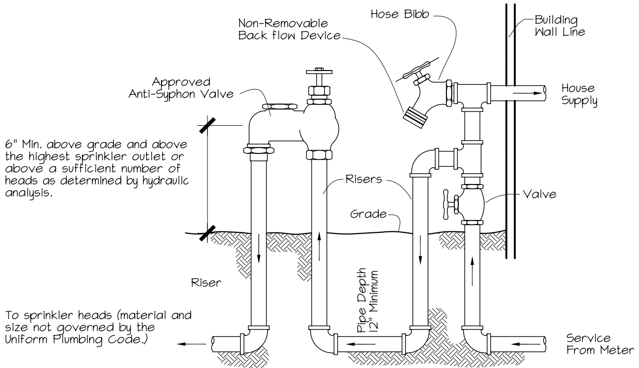
TYPICAL MANIFOLD HOOKUP
