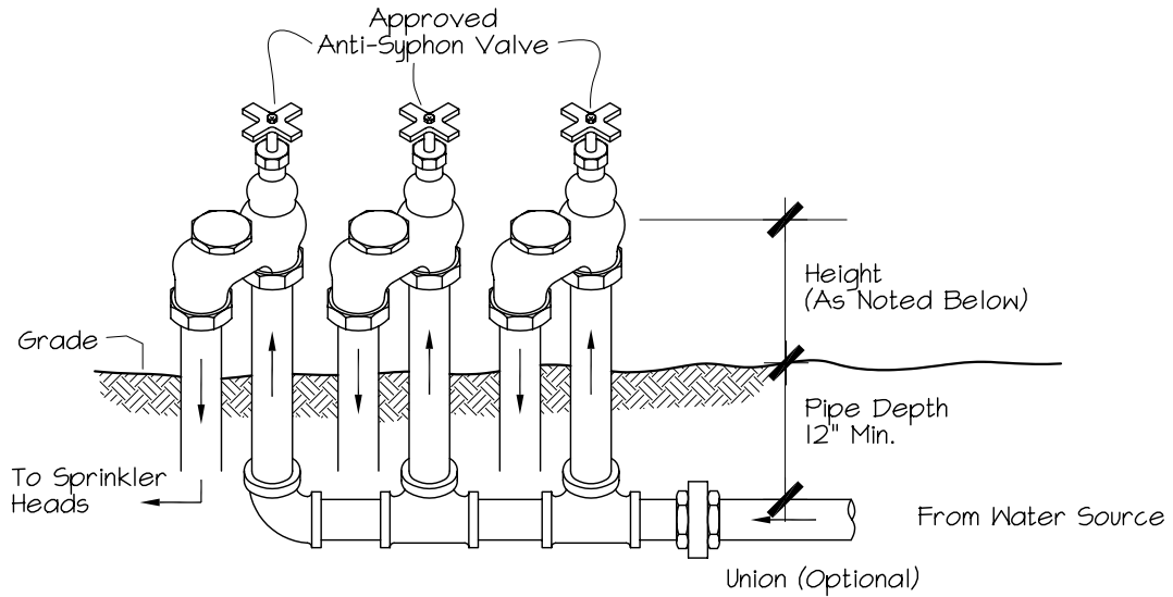
TYPICAL MANIFOLD HOOKUP
